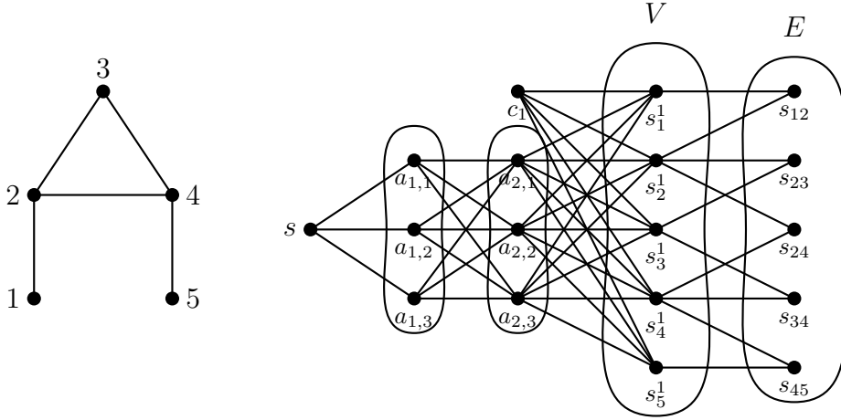
Figure 2: An instance of k -CLIQUE and the corresponding graph G' constructed in the proof of Theorem 2.1 for k = 3 and b = 1 .
