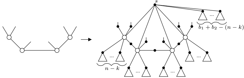
Figure 3: The construction of G' from G in the proof of Theorem 3.1. Added vertices are black and a triangle represents a busy gadget.
