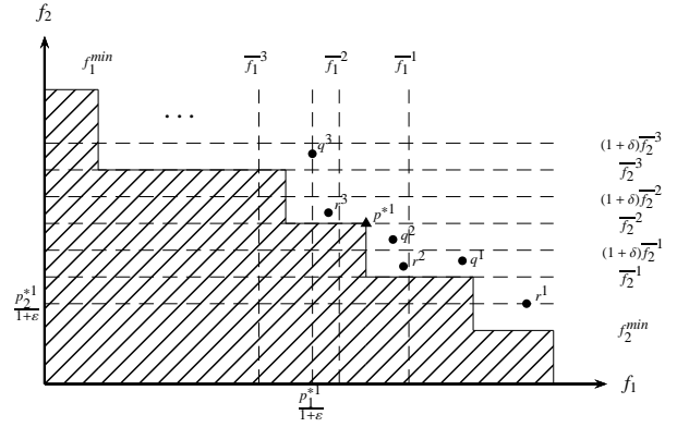
Figure 1: Illustration of Algorithm 1 with 1 + \delta = \sqrt[3]{1 + \varepsilon}
