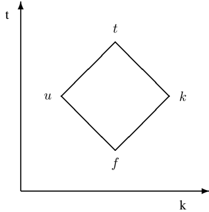
Figure 1. The smallest non trivial interlaced bilattice \Lambda .
