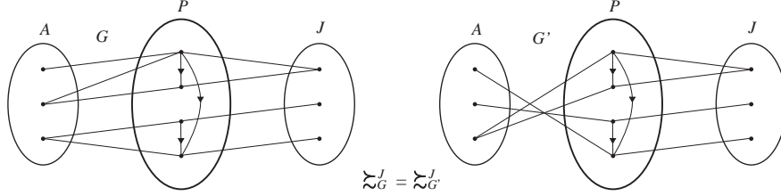
Figure 3: Authors Do Not Matter
