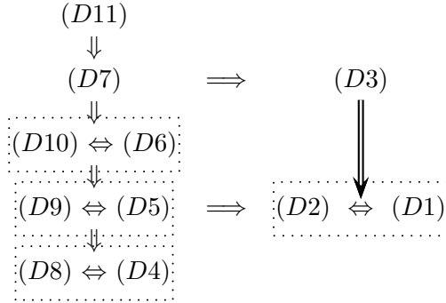
Figure 4. Implication between models resulting from theorem 5.7
