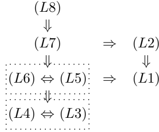
Figure 2. Implication between models resulting from theorem 4.7
