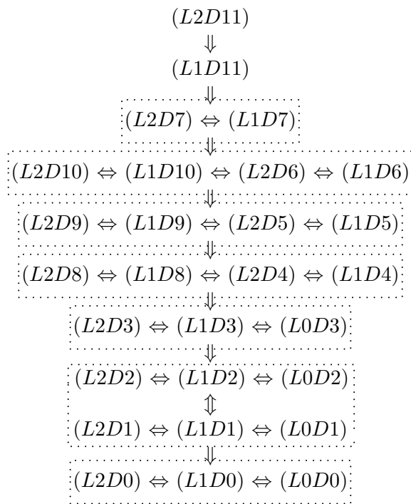
Figure 5. Implication between models resulting from theorems 6.8 and 6.11
