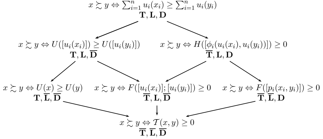
Figure 6. Summary of models
