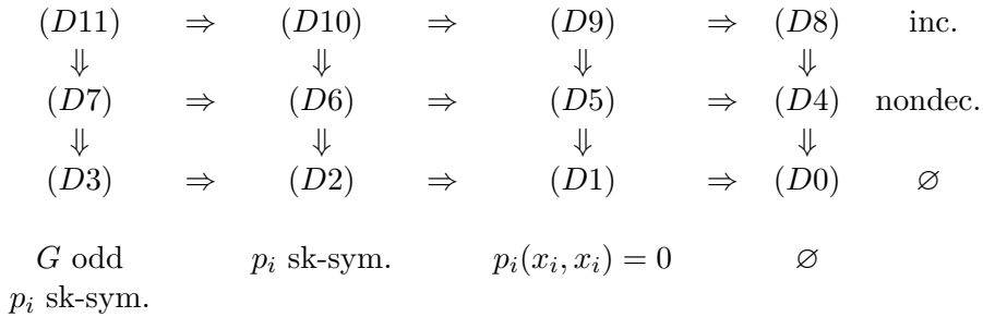
Figure 3. Implication between models involving traces on differences
