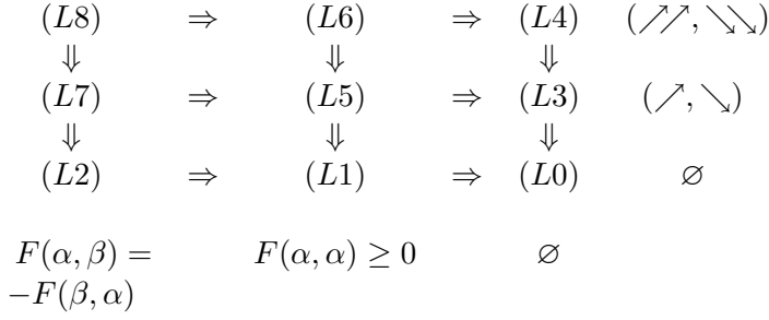
Figure 1. Implication between models involving traces on levels
