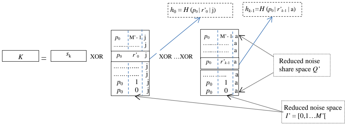
Fig. 4. (k+1) -share noised secret sharing with discount code vector d = d = (d_0 \dots d_{k-1}) = (j \dots a) .
