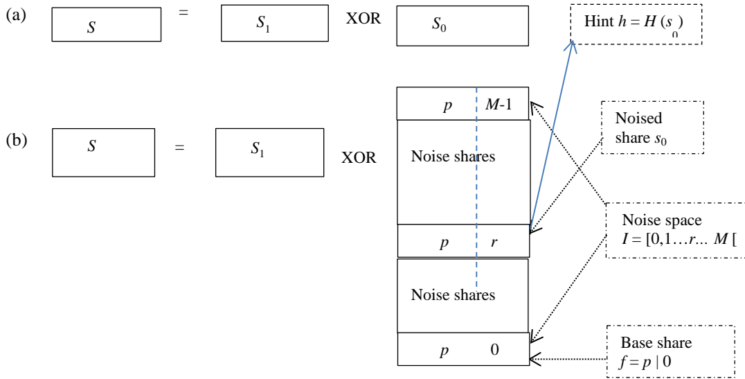
Fig. 1 Secret Sharing (a) and Noised Secret Sharing (b)
