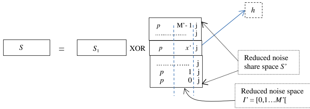
Fig. 2 Reduced noise share and noise spaces for discount code d = 'j' .
