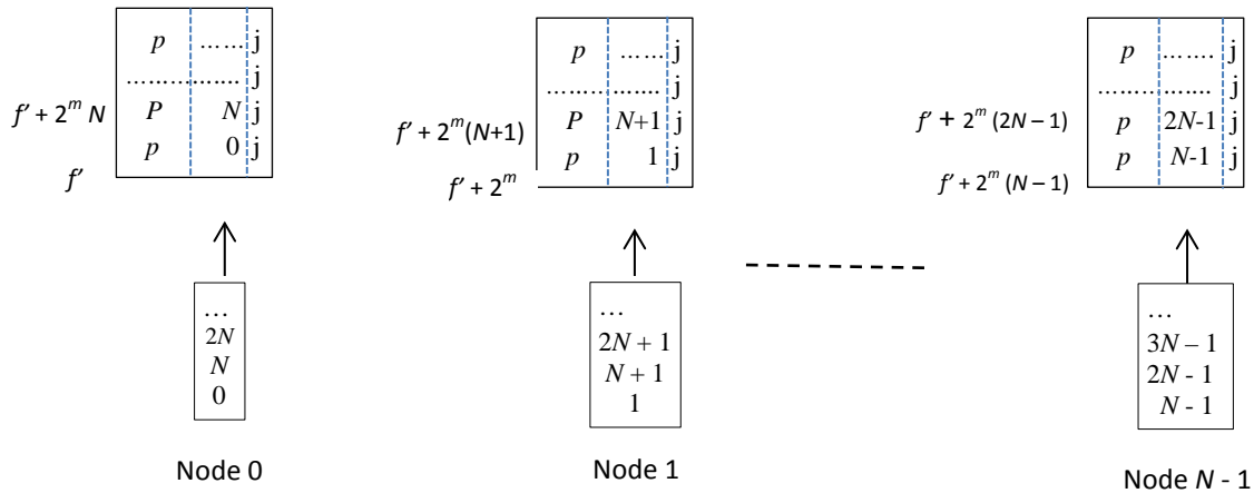
Fig. 3 Distributed partitioned noise and noise share spaces for discounted recovery using the static scheme and discount code 'j' . Node subspace size is M' \setminus N or M' \setminus N + 1 .
