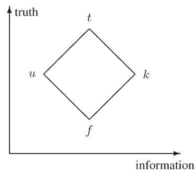
Fig. 1. The bi-lattice suggested by Belnap.
