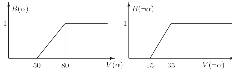
Fig. 2. B(\alpha) and B(\neg\alpha) for Example 2.
