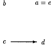
Figure 3: the result of a direct conventional aggregation of the five partial orders
