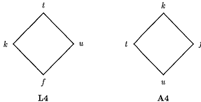
Figure 1. The L4 and A4 lattices.
