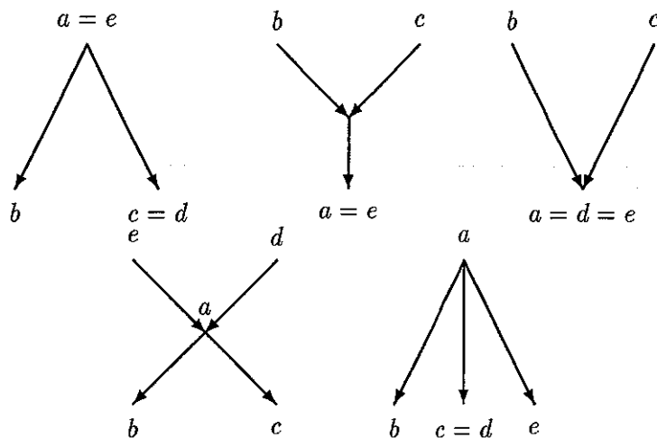
Figure 2: five partial orders that have to be aggregated
