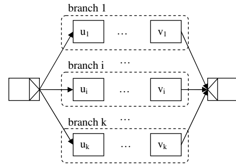
Fig. 2. Complex XOR pattern with interlaced patterns
