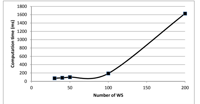
Fig. 8. Computation time for 50-activities workflow with T = 1.5T^* and P = 0.5
