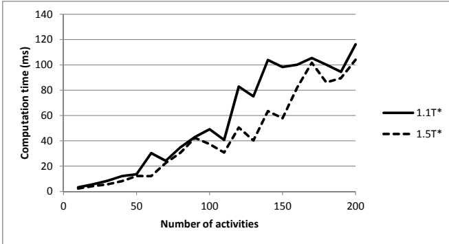
Fig. 6. Computation time for 100 WS per activity
