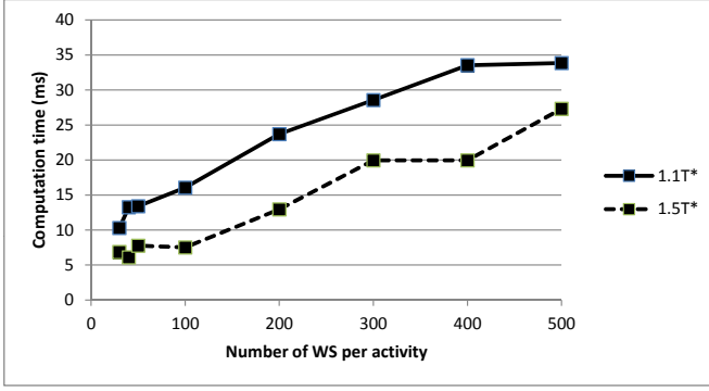
Fig. 5. Computation time for 50-activities workflows
