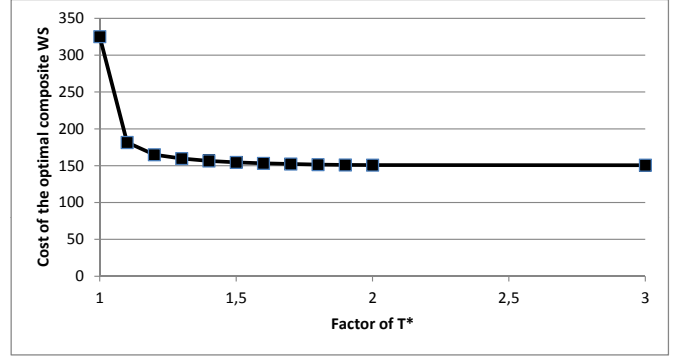
Fig. 7. Cost of the optimal composite WS in function of T
