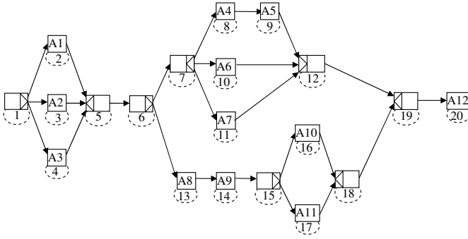
Fig. 3. Example of graph associated with a workflow
