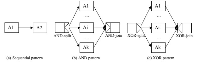
Fig. 1. Workflow patterns
