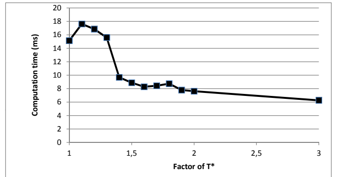
Fig. 4. Computation time in function of the QoS time constraint
