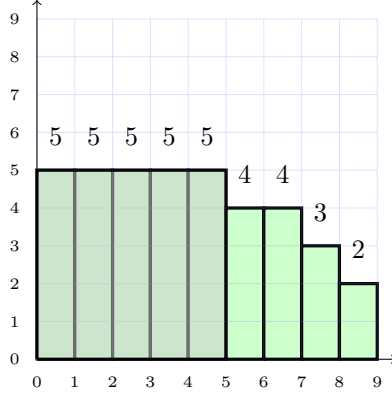
Figure 3: Geometrical interpretation of C14 Square rightwards. We have 5\mathbf{1}_5 \succsim 5\mathbf{1}_5 + \mathbf{1}_4 + \mathbf{1}_4 + \mathbf{1}_3 + \mathbf{1}_2 .
