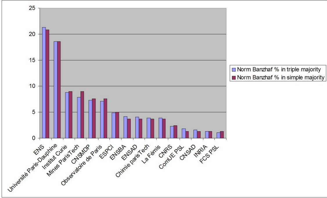
Figure 1: Comparison of the normalized Banzhaf index of the “ideal” triple-majority game v^t (left column) and the Banzhaf index of the weighted majority game v^w (right column) for each Institution of the ComUE .
