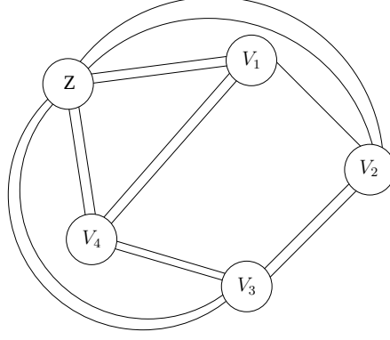
Figure 3: An SP-node-partition configuration for k = 5 and Z = 2
