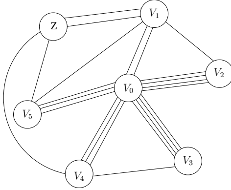
Figure 2: An F -node-partition configuration for k = 5
