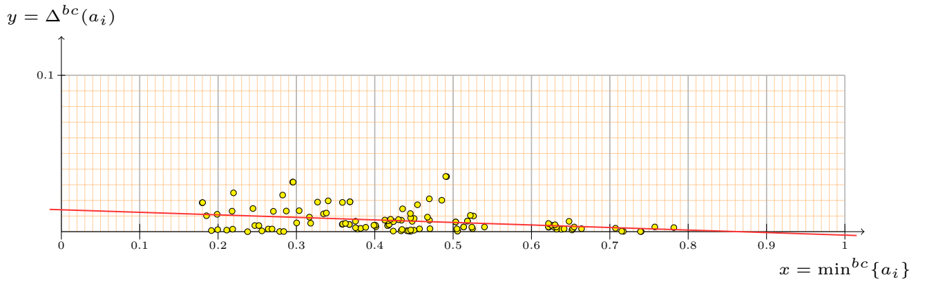
Figure 2: Regression line for the points (\min^{bc}\{a_i\}, \Delta^{bc}(a_i)) : y = -0.0162x + 0.014
