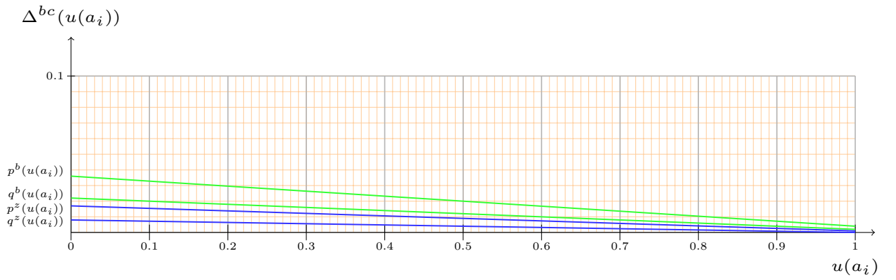
Figure 3: Indifference and preference thresholds lines
