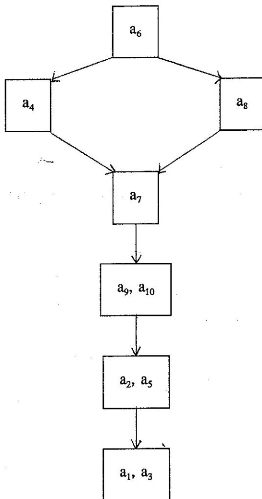
Fig. 5. Priority order of users \hat{O}_p resulting from ELECTRE III
