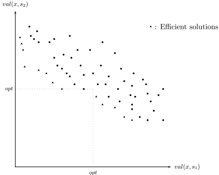
Figure 3: Relationships between min-max and multi-objective versions
