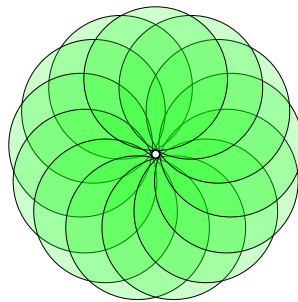
■ Figure 5 A disk realization of the complement of an odd cycle with unit disks as described by Atminas and Zamaraev [4]. Unfortunately, we cannot use this representation.
