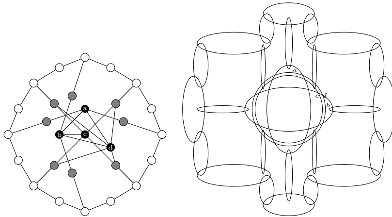
■ Figure 9 A graph G and its representation with empty ellipses.
