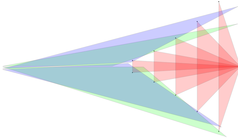
■ Figure 10 A co-2-subdivision of a graph with 5 vertices (in red) represented with triangles. We only represented two edges: one between vertices 1 and 4 (in green), and one between vertices 2 and 3 (in blue). We only represented the points p_1 to p_5 and q_1 to q_5 , and x .
