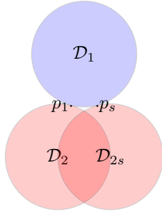
(a) Three important disks with the same size \mathcal{D}_1 , \mathcal{D}_2 , \mathcal{D}_{2s} .
