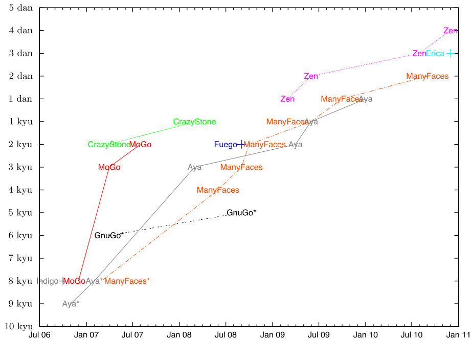
Fig. 8. Ranks of various Go programs discussed in the text on the Kiseido Go Server (KGS). Each point represents the first date at which a program held the given rank for 20 consecutive games on KGS. Note that each program plays with different time controls, which may cause variations in rank; and that some programs play more regularly than others, which may cause variations in date. 18
