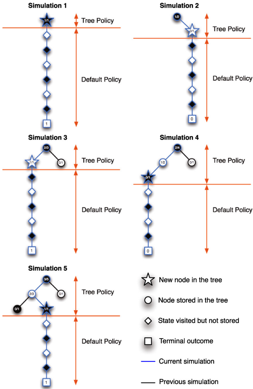
Fig. 1. Five simulations of a simple Monte-Carlo tree search. Each simulation has an outcome of 1 for a black win or 0 for a white win (square). At each simulation a new node (star) is added into the search tree. The value of each node in the search tree (circles and star) is then updated to count the number of black wins, and the total number of visits (wins/visits).
