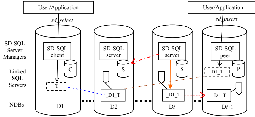
Fig. 1. SD-SQL Server Architecture
