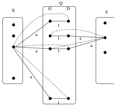
■ Figure 1 An illustration of the reduction.
