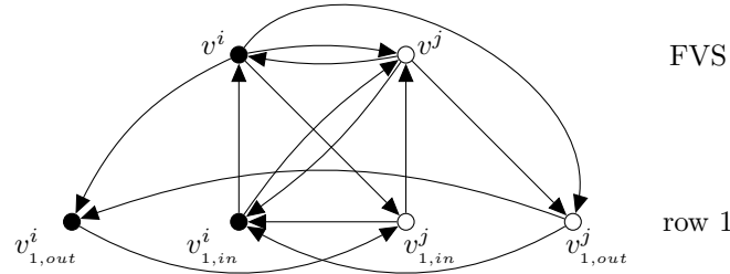
■ Figure 2 Graph showing the connections between two vertices of the clique palette ( v^i, v^j , where i < j ) and the corresponding vertices of row 1.
