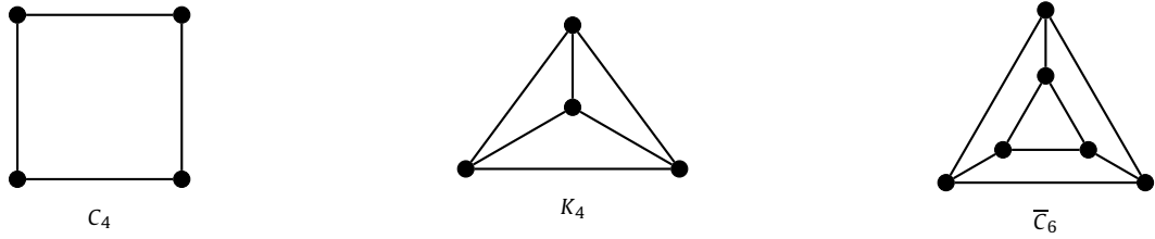
Fig. 1. From left to right: the brace C_4 , which is the smallest solid bipartite graph; the brick K_4 , which is the smallest solid nonbipartite graph; the brick \bar{C}_6 , which is the smallest nonsolid brick.
